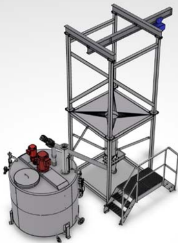
ChemiMix BTL-3000-750-T-00
